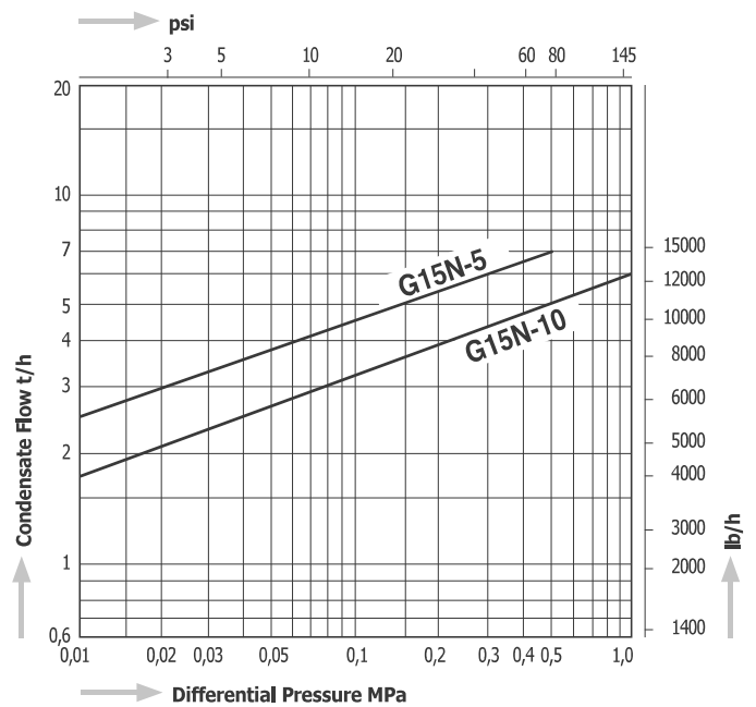
Capacity Chart G15N
