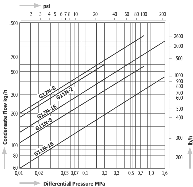
Capacity Chart G11N, G12N
